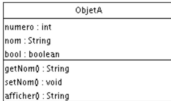
FIGURE II.3.2. – Classe en UML
