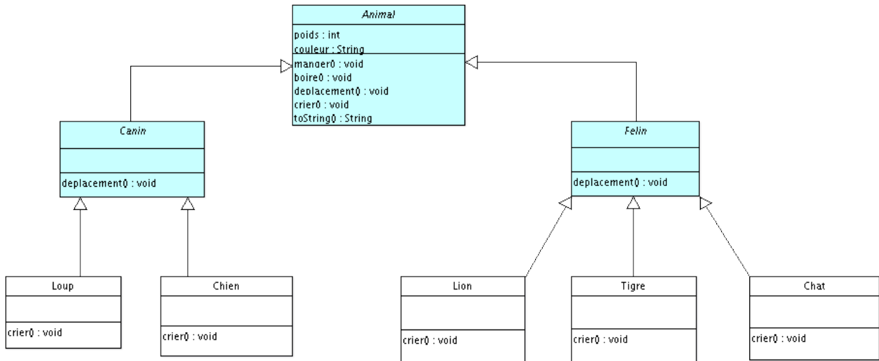
FIGURE II.5.3. – Nouvelle architecture des classes
